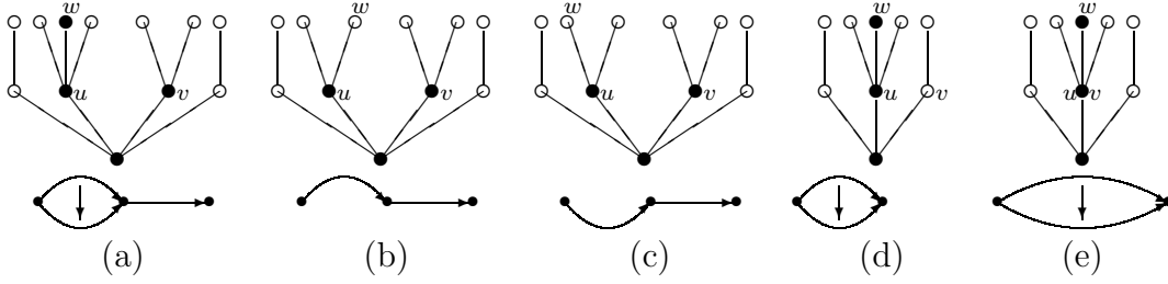
Figure 8: The duality. In the upper row, \bullet denotes an interior element and \circ an endpoint of a fibre, and the labels u, v, w show what the coface maps ‘ \phi ’ do
