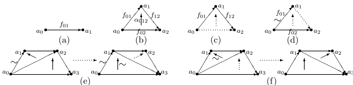
Figure 9: (a) Element of A[1] , with, for instance, the \{0\} -face labelled a_0 ; (b) element of A[2] ; (c) (admissible) horn \Lambda_2^1 \longrightarrow A ; (d) admissible horn \Lambda_2^0 \longrightarrow A , with \sim indicating a hollow face; (e) admissible horn \Lambda_3^0 \longrightarrow A , with labels f_{ij}, \alpha_{ijk} omitted; (f) as (e), but for \Lambda_3^1 .
