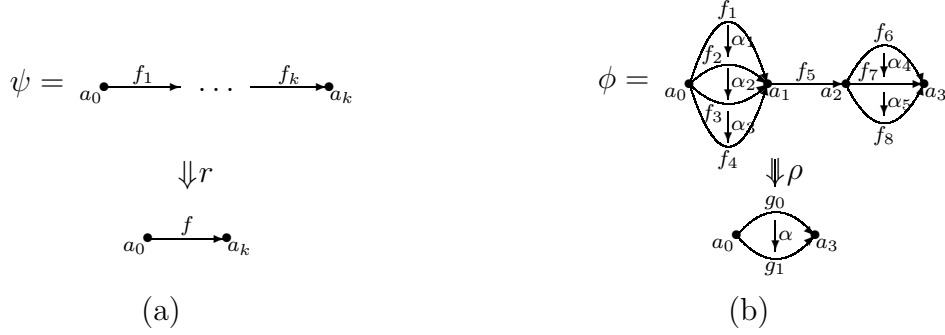
Figure 6: (a) A 1-cell, and (b) a typical 2-cell, of R . Here a_i, f_i, f, g_i, \alpha_i and \alpha are all cells of A
