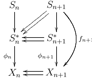
Figure 6: universal property
